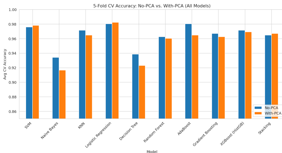
Figure 3: 5-fold CV accuracy comparison: No-PCA vs. With-PCA, all 10 models
