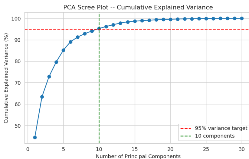
Figure 1: PCA scree plot – cumulative explained variance vs. number of components
