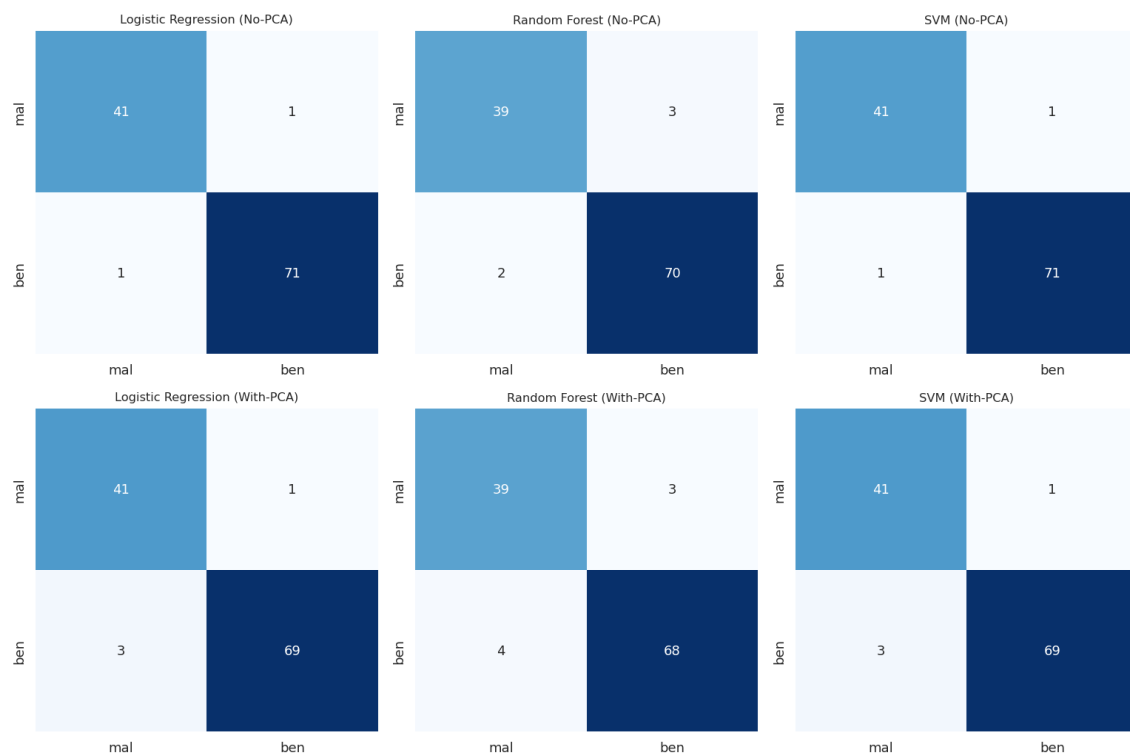
Figure 5: Confusion matrices for selected models – top row: No-PCA, bottom row: With-PCA
