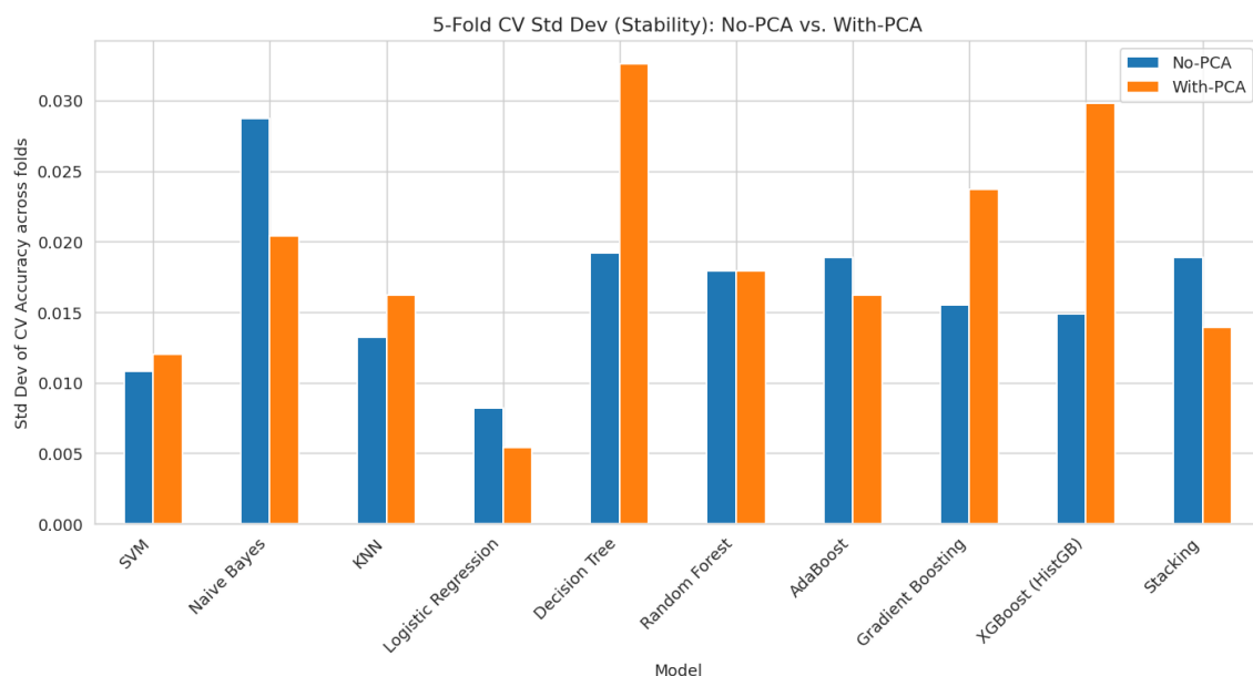
Figure 4: 5-fold CV standard deviation (stability) comparison: No-PCA vs. With-PCA
