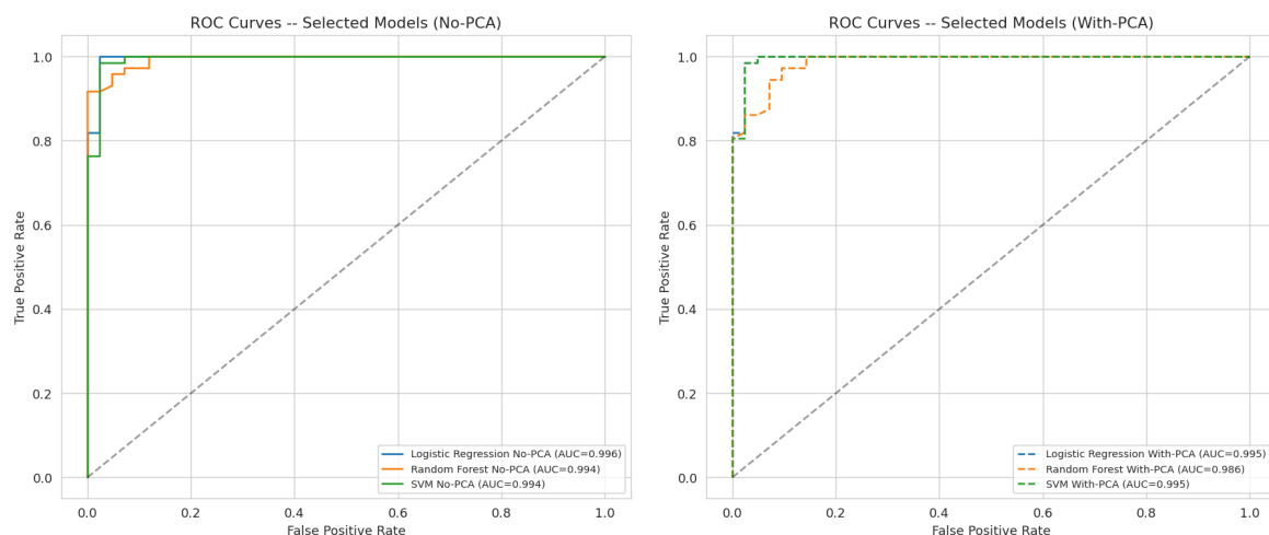
Figure 6: ROC curves for selected models – No-PCA (left) vs. With-PCA (right)
